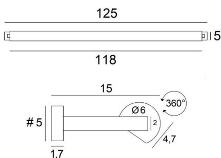
ALEXANDRIE 120 in brushed bronze. Metal finish code: 29
