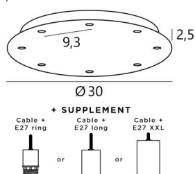
CEILING BASE 8 o30 in light bronze. Metal finish code: 28. Optional: a wide choice of cables and fittings (+supplement)
