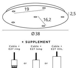
CEILING BASE 6 o38 in structured black. Metal finish code: 02. Optional: a wide choice of cables and fittings (+supplement)
