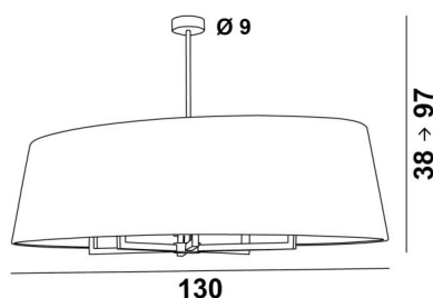
TOURAH 6 OVALE in brushed bronze with oval lampshade L130cm in Plissé Or (fabric from category 4)
