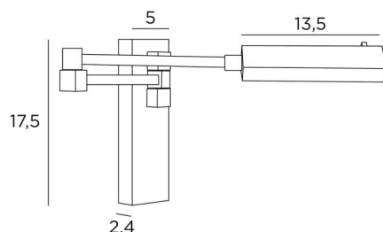
VESTA without switch in brushed bronze
