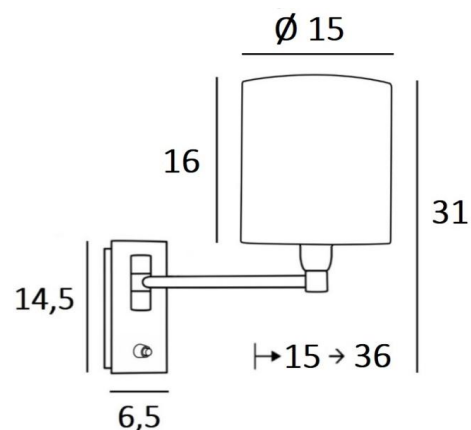
SOKARIS +SW in brushed bronze with lampshade in Tilia Starry Blue (fabric from category 5)
